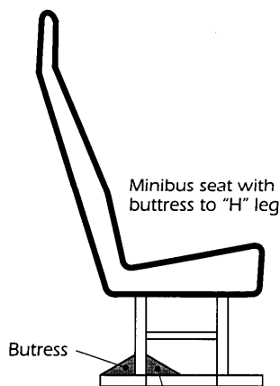
Typical Minibus seat with standard "H" leg
